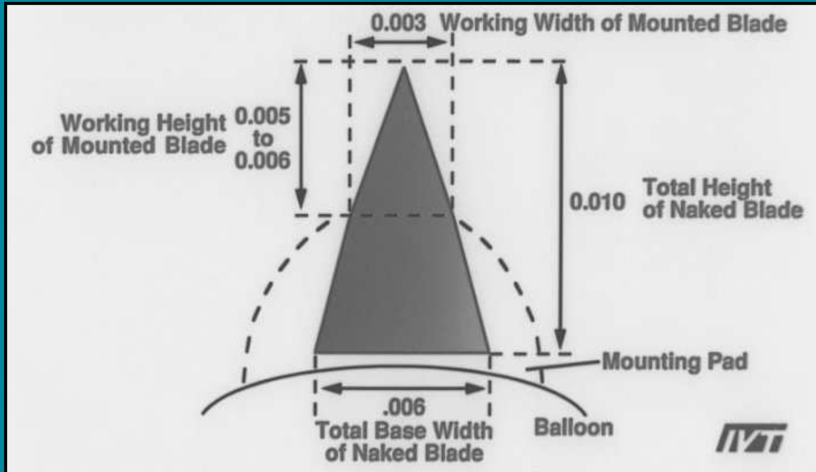
Atherotome dimensions
